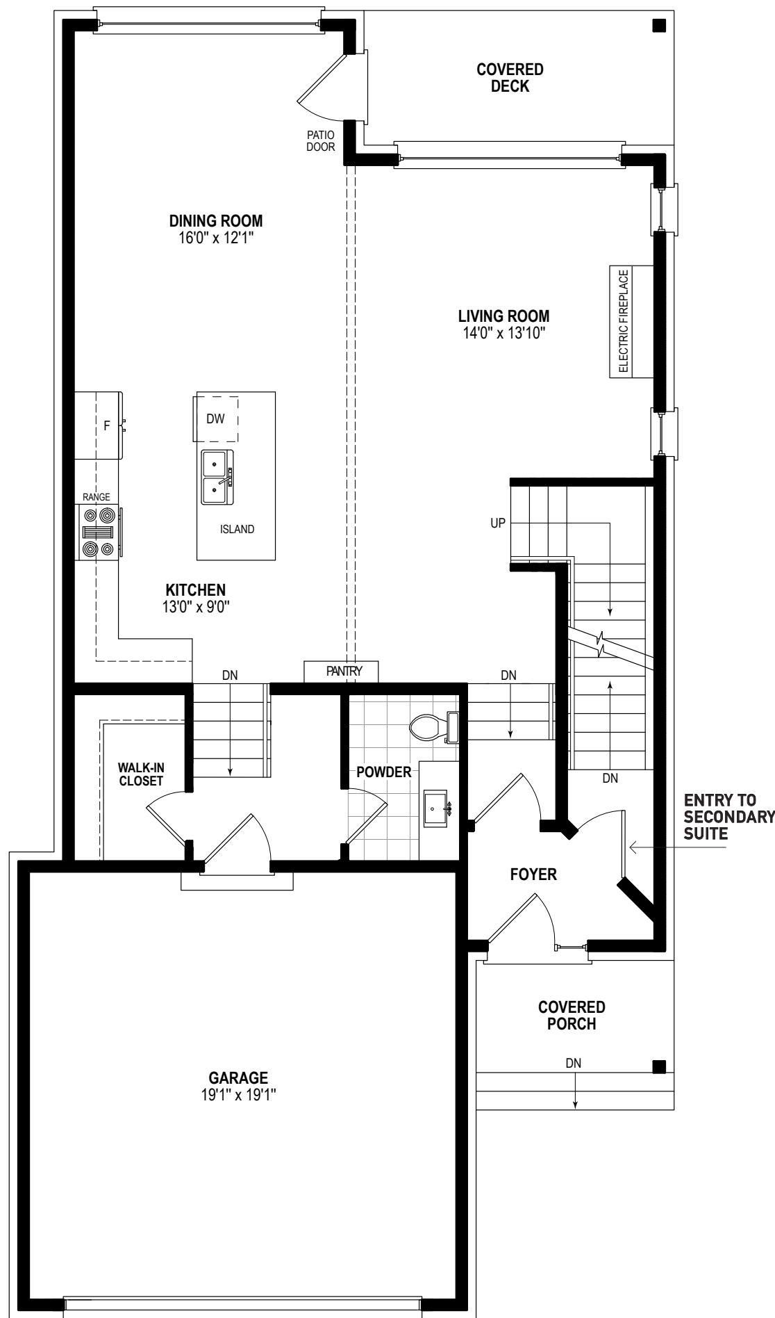
GROUND FLOOR WITH SECONDARY SUITE
